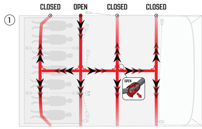
1 SINGLE POINT INFLATION: OPERATE SELECTED VALVE AND KEEP ALL CONNECTING TUBES OPEN
